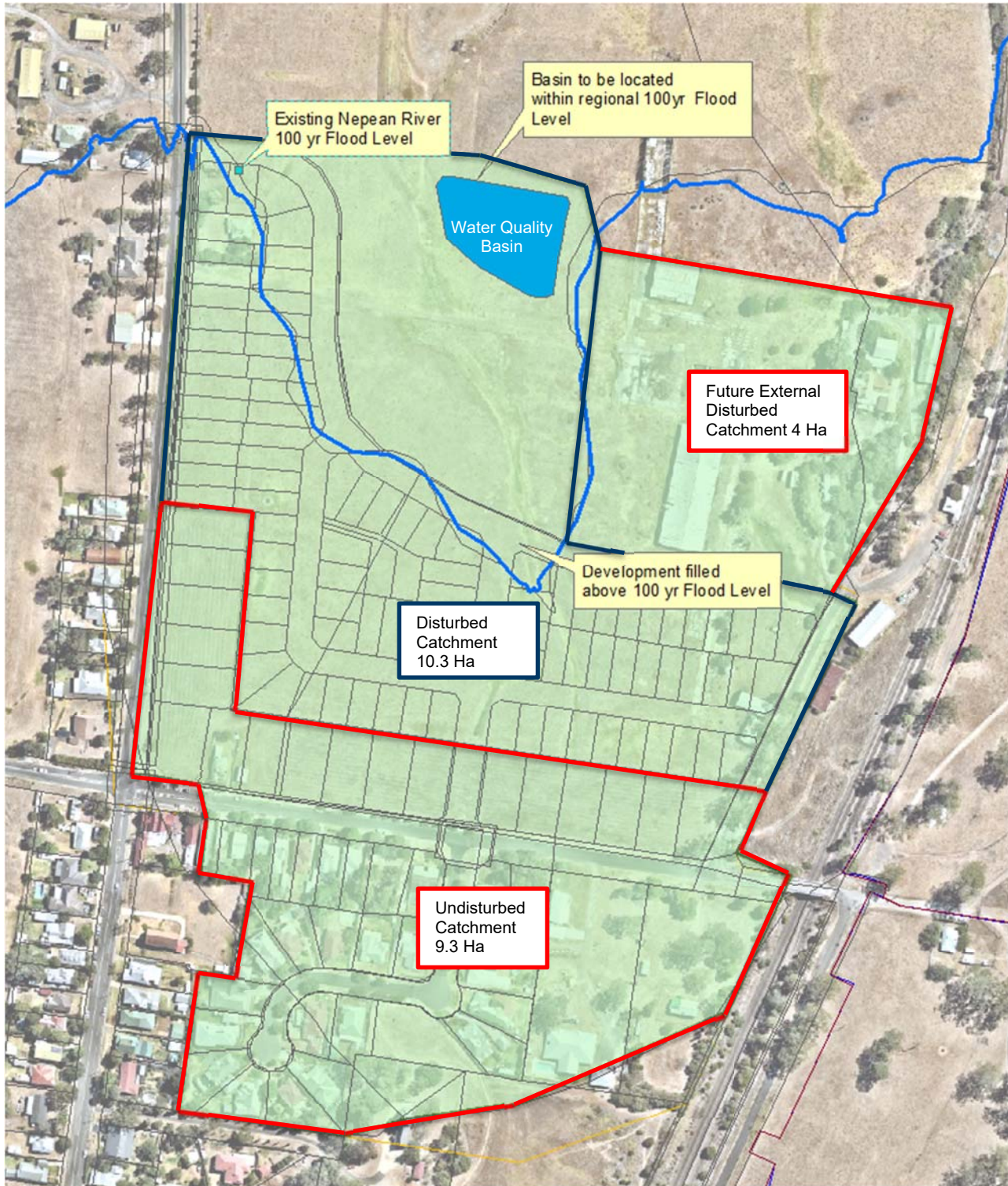
Figure 3 – Catchment Plan
